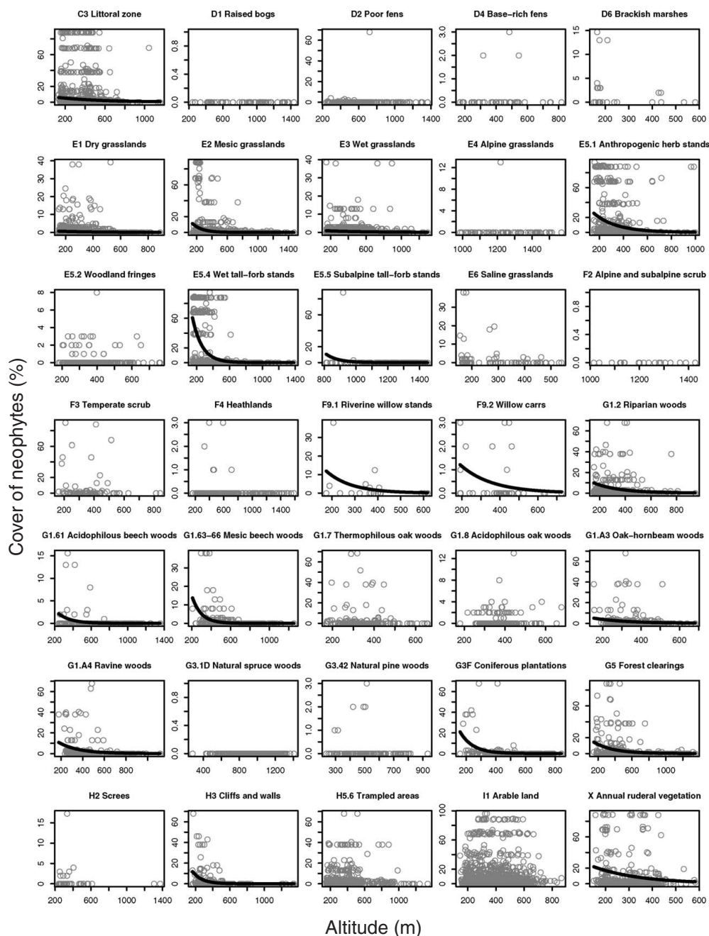
Fig. 4. – Relationships between the level of invasion by neophytes, measured as the total percentage covers of neophytes in vegetation plots, and altitude for particular habitats. Curves are fitted using generalized linear models (log link function and Poisson distribution of errors) for those habitats where the relationship was significant. See Table 2 for model statistics.
